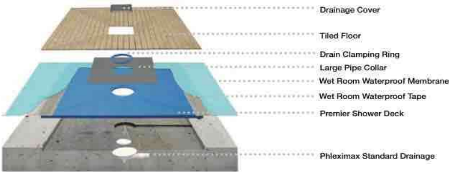
Concrete Installation
