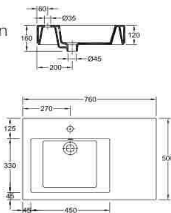
Left hand illustrated
