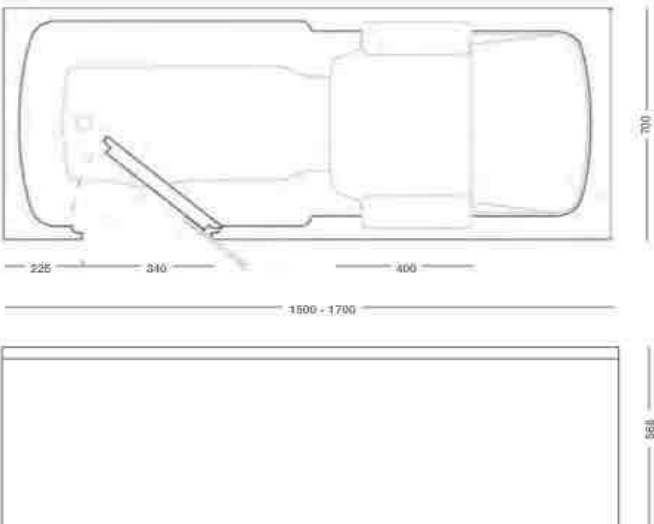
Left hand illustrated
