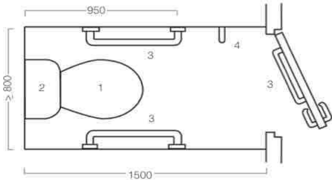
B) Plan (New Building)
