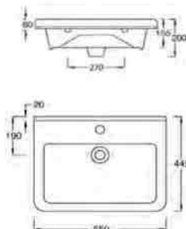
Can be mounted on adjustable height assemblies, use P6810645 bolts.
