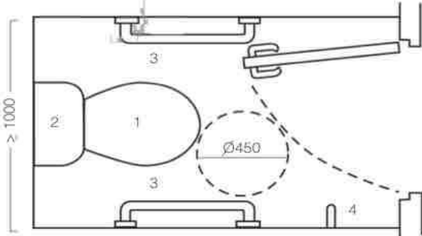
C) Plan (Existing Building)
