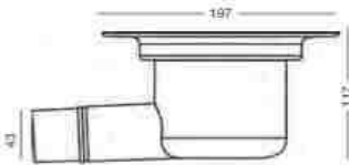
Shower Gully P6820599
