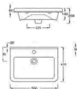
Can be mounted on adjustable height assemblies, use P6810645 bolts.
