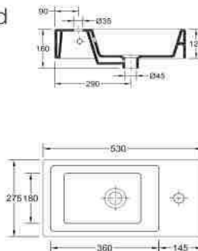
Left hand illustrated
